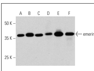
emerin (A-5): sc-515522. Western blot analysis of emerin expression in Hep G2 (A), MCF7 (B), RT-4 (C), A-431 (D), U-698-M (E) and MDA-MB-435S (F) whole cell lysates.
