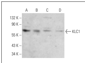
KLC1 (H-7): sc-515792. Western blot analysis of KLC1 expression in IMR-32 (A), BE (2)-M17 (B), C2C12 (C) and A-10 (D) whole cell lysates.
