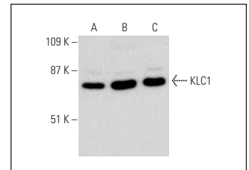
KLC1 (H-7): sc-515792. Western blot analysis of KLC1 expression in IMR-32 (A), SK-N-SH (B) and SH-SY5Y (C) whole cell lysates.
