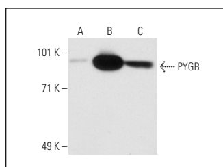
PYGB/M (3G1): sc-51925. Western blot analysis of PYGB expression in non-transfected 293T: sc-117752 (A), human PYGB transfected 293T: sc-113669 (B) and Hep G2 (C) whole cell lysates.
