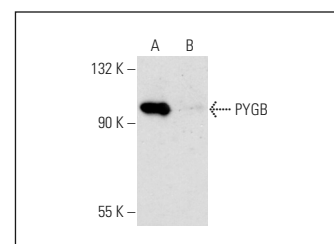
PYGB/M (3G1): sc-51925. Western blot analysis of PYGB expression in human PYGB transfected: sc-111195 (A) and non-transfected: sc-110760 (B) Hep G2 293 whole cell lysates.
