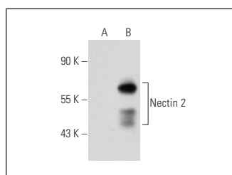
Nectin 2 (502-57): sc-52708. Western blot analysis of Nectin 2 expression in non-transfected: sc-117752 (A) and mouse Nectin 2 transfected: sc-127214 (B) 293T whole cell lysates.
