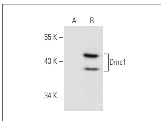
Dmc1 (1D12/4): sc-53268. Western blot analysis of Dmc1 expression in non-transfected: sc-117752 (A) and human Dmc1 transfected: sc-128471 (B) 293T whole cell lysates.
