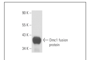
Dmc1 (1D12/4): sc-53268. Western blot analysis of human recombinant DMC-1 fusion protein.
