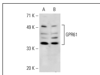
GPR61 (D-14): sc-54600. Western blot analysis of GPR61 expression in IMR-32 (A) and SK-N-SH (B) whole cell lysates.
