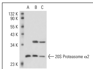
20S Proteasome \alpha 2 (S-16): sc-54671. Western blot analysis of 20S Proteasome \alpha 2 expression in Jurkat (A), JAR (B) and JEG-3 (C) whole cell lysates.
