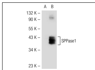
SPPase1 (G-20): sc-55305. Western blot analysis of SPPase1 expression in non-transfected: sc-117752 (A) and mouse SPPase1 transfected: sc-123749 (B) 293T whole cell lysates.
