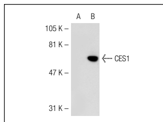
CES1 (S-16): sc-55921. Western blot analysis of CES1 expression in non-transfected: sc-117752 (A) and human CES1 transfected: sc-111916 (B) 293T whole cell lysates.
