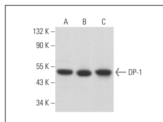
DP-1 (SPM178): sc-56526. Western blot analysis of DP-1 expression in Raji (A) and 3T3-L1 (B) whole cell lysates and A-431 nuclear extract (C).
