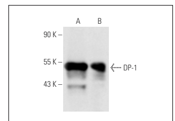
DP-1 (SPM178): sc-56526. Western blot analysis of DP-1 expression in Raji (A) and HeLa (B) whole cell lysates.
