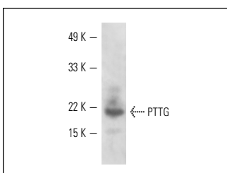
PTTG (T-20): sc-5842. Western blot analysis of PTTG expression in rat pituitary tissue extract.
