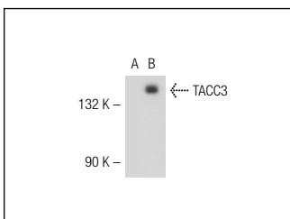
TACC3 (S-18): sc-5887. Western blot analysis of TACC3 expression in non-transfected: sc-117752 (A) and human TACC3 transfected: sc-111721 (B) 293T whole cell lysates.
