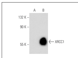
XRCC1 (D-18): sc-5902. Western blot analysis of XRCC1 expression in non-transfected: sc-117752 (A) and mouse XRCC1 transfected: sc-127792 (B) 293T whole cell lysates.
