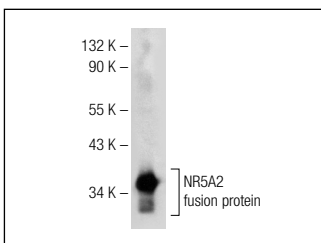
NR5A2 (V-14): sc-5998. Western blot analysis of human recombinant NR5A2 fusion protein.
