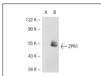
ZPR1 (C-20): sc-6140. Western blot analysis of ZPR1 expression in non-transfected: sc-117752 (A) and mouse ZPR1 transfected: sc-124831 (B) 293T whole cell lysates.
