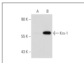
Krs-1 (N-19): sc-6212. Western blot analysis of Krs-1 expression in non-transfected: sc-110760 (A) and human Krs-1 transfected: sc-111111 (B) 293 whole cell lysates.
