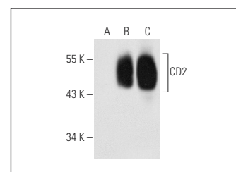
CD2 (UMCD2): sc-65247. Western blot analysis of CD2 expression in non-transfected 293T: sc-117752 (A), human CD2 transfected 293T: sc-172563 (B) and Jurkat (C) whole cell lysates.
