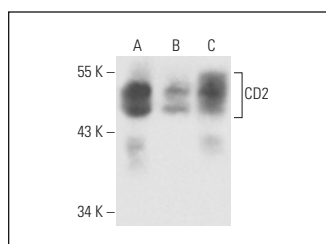
CD2 (UMCD2/IE7E8): sc-65247. Western blot analysis of CD2 expression in CCRF-CEM (A), HuT 78 (B) and human PBL (C) whole cell lysates.
