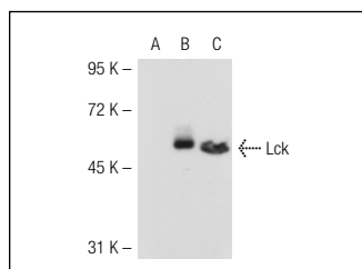
Lck (8E5F9): sc-65506. Western blot analysis of Lck expression in non-transfected 293T: sc-117752 (A), mouse Lck transfected 293T: sc-125538 (B) and HuT 78 (C) whole cell lysates.
