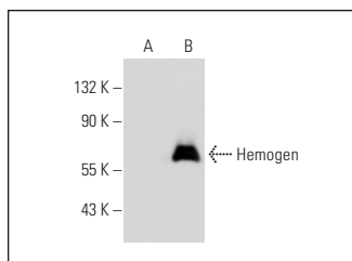
Hemogen (G-17): sc-66235. Western blot analysis of Hemogen expression in non-transfected: sc-117750 (A) and human Hemogen transfected: sc-115998 (B) whole cell lysates.
