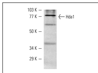
Hda1 (yC-20): sc-6657. Western blot analysis of Hda1 expression in S. cerevisiae whole cell lysate.
