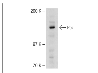
Pez (G-20): sc-66616. Western blot analysis of Pez expression in HUV-EC-C whole cell lysate.
