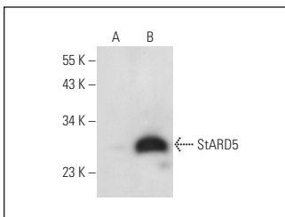
StARD5 (C-20): sc-66664. Western blot analysis of StARD5 expression in non-transfected: sc-117752 (A) and mouse StARD5 transfected: sc-127598 (B) 293T whole cell lysates.
