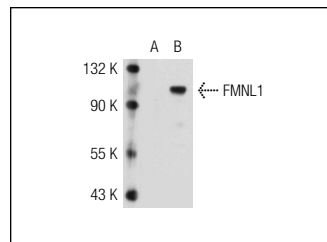
FMNL1 (F-15): sc-66758. Western blot analysis of FMNL1 expression in non-transfected: sc-117752 (A) and human FMNL1 transfected: sc-113684 (B) 293T whole cell lysates.
