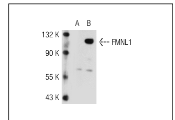
FMNL1 (P-17): sc-66760. Western blot analysis of FMNL1 expression in non-transfected: sc-117752 (A) and human FMNL1 transfected: sc-113684 (B) 293T whole cell lysates.
