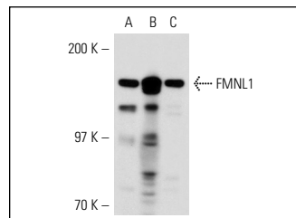
FMNL1 (P-17): sc-66760. Western blot analysis of FMNL1 expression in Jurkat (A), NK-92 (B) and HUT 78 (C) whole cell lysates.
