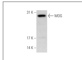
MOG (H-72): sc-66968. Western blot analysis of MOG expression in 293T whole cell lysate.
