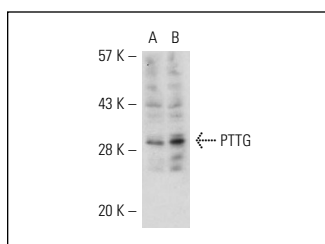
PTTG (S-19): sc-67817. Western blot analysis of PTTG expression in Jurkat (A) and MOLT-4 (B) whole cell lysates.
