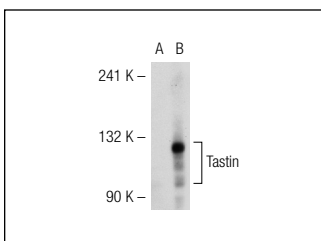
Tastin (S-15): sc-67873. Western blot analysis of Tastin expression in non-transfected: sc-117752 (A) and human Tastin transfected: sc-115239 (B) 293T whole cell lysates.
