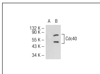
Cdc40 (F-20): sc-68266. Western blot analysis of Cdc40 expression in non-transfected: sc-117752 (A) and human Cdc40 transfected: sc-111958 (B) 293T whole cell lysates.
