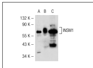
INSM1 (H-45): sc-68355. Western blot analysis of INSM1 expression in non-transfected 293T: sc-117752 (A), mouse INSM1 transfected 293T: sc-127011 (B) and TT (C) whole cell lysates.
