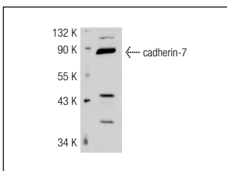
cadherin-7 (H-47): sc-68422. Western blot analysis of cadherin-7 expression in DU 145 whole cell lysate.
