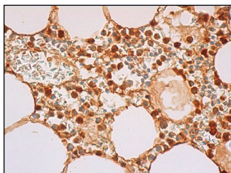
MLL5 (L-14): sc-68635. Immunoperoxidase staining of formalin fixed, paraffin-embedded human bone marrow tissue showing cytoplasmic and nuclear staining of hematopoietic cells.
