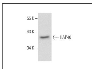
HAP40 (P-19): sc-69489. Western blot analysis of HAP40 expression in 293T whole cell lysate.
