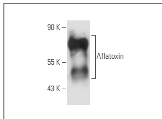
Aflatoxin (AFC-7): sc-69862. Western blot analysis of recombinant Aflatoxin.
