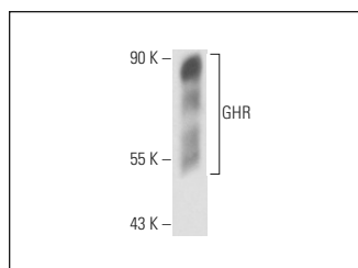
GHR (MAB 1): sc-69883. Western blot analysis of human recombinant truncated GHR under reducing conditions.
