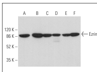
Ezrin (4i251): sc-71080. Western blot analysis of Ezrin expression in F9 (A), Daudi (B), AN3 CA (C), HT-29 (D), C2C12 (E) and MCF7 (F) whole cell lysates.
