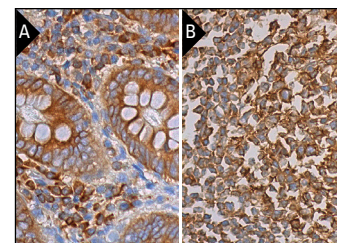
Ezrin (4i251): sc-71080. Immunoperoxidase staining of formalin fixed, paraffin-embedded human appendix tissue showing cytoplasmic and membrane staining of glandular cells and lymphoid cells (A). Immunoperoxidase staining of formalin fixed, paraffin-embedded human lymph node tissue showing cytoplasmic and membrane staining of cells in germinal center and cells in non-germinal center (B).
