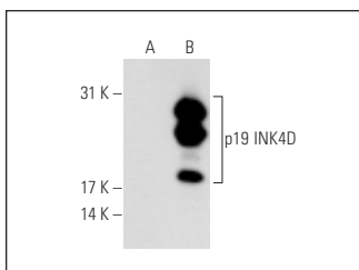
p19 INK4D (0.N.485): sc-71807. Western blot analysis of p19 INK4D expression in non-transfected: sc-117752 (A) and human p19 INK4D transfected: sc-174520 (B) 293T whole cell lysates.
