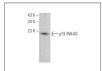
p19 INK4D (0.N.485): sc-71807. Western blot analysis of p19 INK4D expression in Jurkat whole cell lysate.
