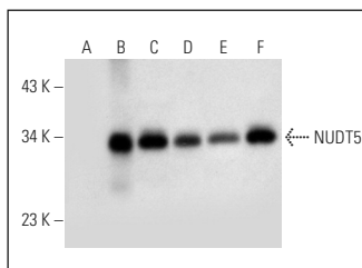
NUDT5 (P-18): sc-74757. Western blot analysis of NUDT5 expression in non-transfected 293T: sc-117752 (A), mouse NUDT5 transfected 293T: sc-127247 (B), HeLa (C), Hep G2 (D), U-937 (E) and Jurkat (F) whole cell lysates.
