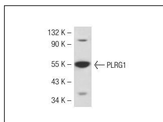
PLRG1 (D-20): sc-74843. Western blot analysis of PLRG1 expression in K-562 nuclear extract.
