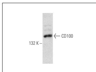
CD100 (S-16): sc-79404. Western blot analysis of CD100 expression in Jurkat whole cell lysate.
