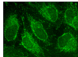
GPR88 (N-13): sc-79515. Immunofluorescence staining of formalin-fixed HeLa cells showing cytoplasmic localization.
