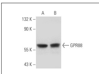
GPR88 (N-13): sc-79515. Western blot analysis of GPR88 expression in Jurkat (A) and IMR-32 (B) whole cell lysates.
