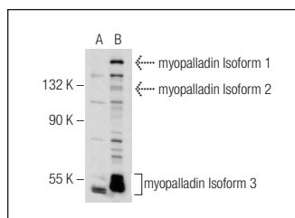
myopalladin (G-19): sc-79638. Western blot analysis of myopalladin expression in HeLa whole cell lysate (A) and HeLa nuclear extract (B).
