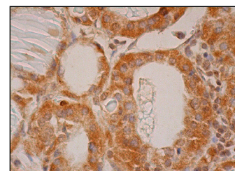
UVRAG (C-18): sc-82115. Immunoperoxidase staining of formalin fixed, paraffin-embedded human thyroid gland tissue showing cytoplasmic staining of glandular cells.
