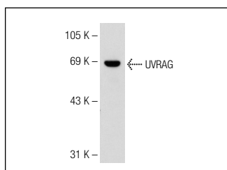
UVRAG (C-18): sc-82115. Western blot analysis of UVRAG expression in MCF7 whole cell lysate.
