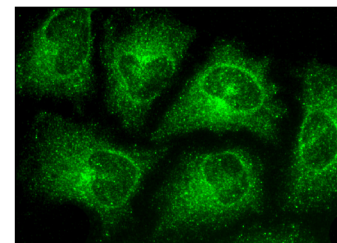
Ces1d (S-13): sc-82555. Immunofluorescence staining of methanol-fixed HeLa cells showing cytoplasmic localization.
