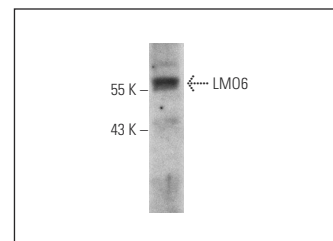
LMO6 (T-19): sc-82651. Western blot analysis of LMO6 expression in MIA PaCa-2 whole cell lysate.
