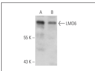
LMO6 (T-19): sc-82651. Western blot analysis of LMO6 expression in HeLa (A) and SK-MEL-24 (B) whole cell lysates.
