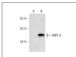
WIPI-4 (K-20): sc-83076. Western blot analysis of WIPI-4 expression in non-transfected: sc-117752 (A) and mouse WIPI-4 transfected: sc-124647 (B) 293T whole cell lysates.
