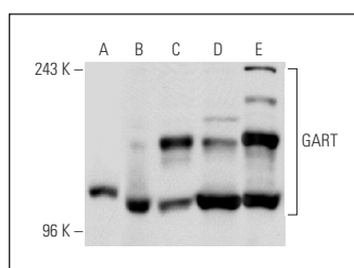
GART (S-20): sc-83255. Western blot analysis of GART expression in 293T (A), A-431 (B), Daudi (C) and K-562 (D) whole cell lysates and HeLa nuclear extract (E).
