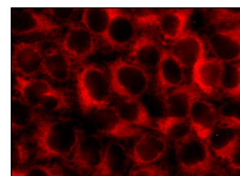
GART (S-20): sc-83255. Immunofluorescence staining of methanol-fixed HeLa cells showing cytoplasmic localization.
