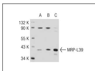
MRP-L39 (I-19): sc-83301. Western blot analysis of MRP-L39 expression in non-transfected 293T: sc-117752 (A), mouse MRP-L39 transfected 293T: sc-121767 (B) and Hep G2 (C) whole cell lysates.
