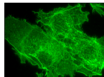
LOC647166 (E-20): sc-84147. Immunofluorescence staining of formalin-fixed Hep G2 cells showing membrane localization.
