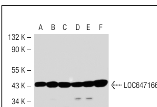
LOC647166 (E-20): sc-84147. Western blot analysis of LOC647166 expression in HEK293 (A), HeLa (B), Hep G2 (C), K-562 (D), SK-N-MC (E) and SHP-77 (F) whole cell lysates.
