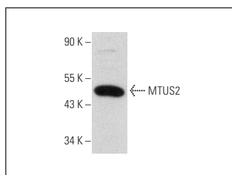
MTUS2 (C-14): sc-84342. Western blot analysis of MTUS2 expression in NIH/3T3 whole cell lysate.
