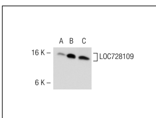
LOC728109 (C-15): sc-85661. Western blot analysis of LOC728109 expression in SH-SY5Y (A), Hep G2 (B) and K-562 (C) whole cell lysates.
